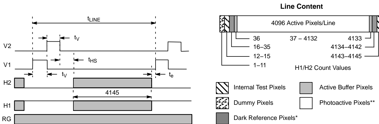
Figure 14. Line Timing
